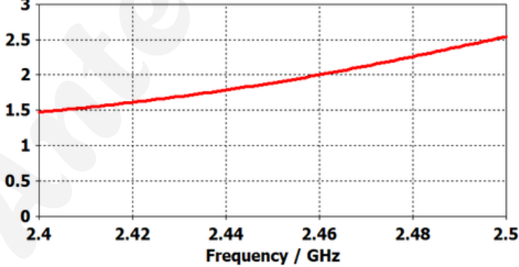
Axial Ratio
